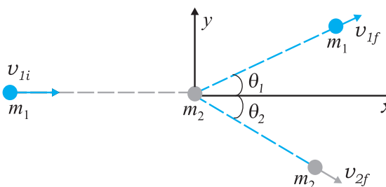
Fig. 5.10 Collision of mass m_1 , with a stationary mass m_2 .
