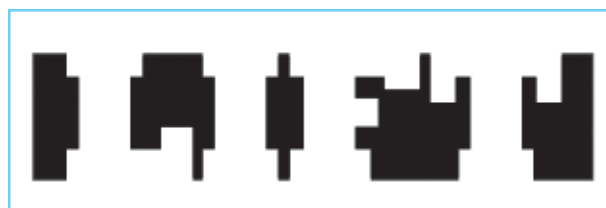
Fig.4.9 : Surroundedness
