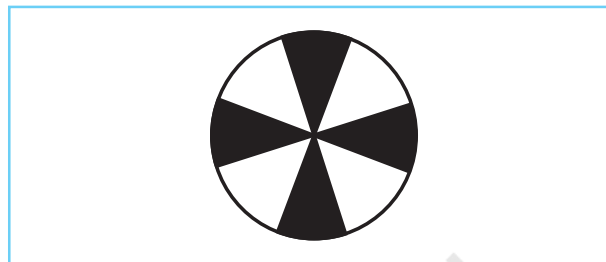
Fig.4.7 : Smallness
