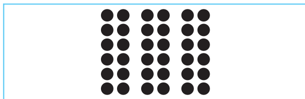
Fig.4.4 : Proximity
